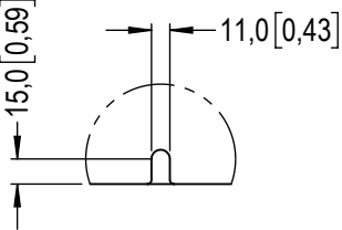
DETALHE B/ DETAIL B ESCALA/SCALE 1 : 5
