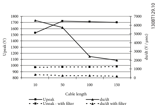
Illustration 3.12 690V - with and du/dt filter
