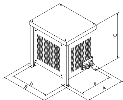
Illustration 5.12 IP23 floor mounted
