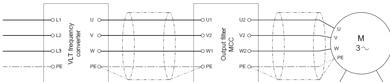
Illustration 5.3 Wiring diagram
