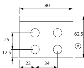
Illustration 5.15 L-shaped terminal kit 130B3139 (Only for du/dt filters)
