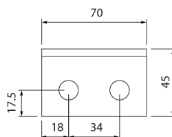
Illustration 5.14 L-shaped terminal kit 130B3138 (Only for du/dt filters)
