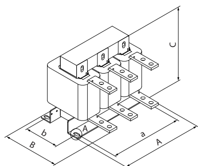
Illustration 5.11 IP00 floor mounted
