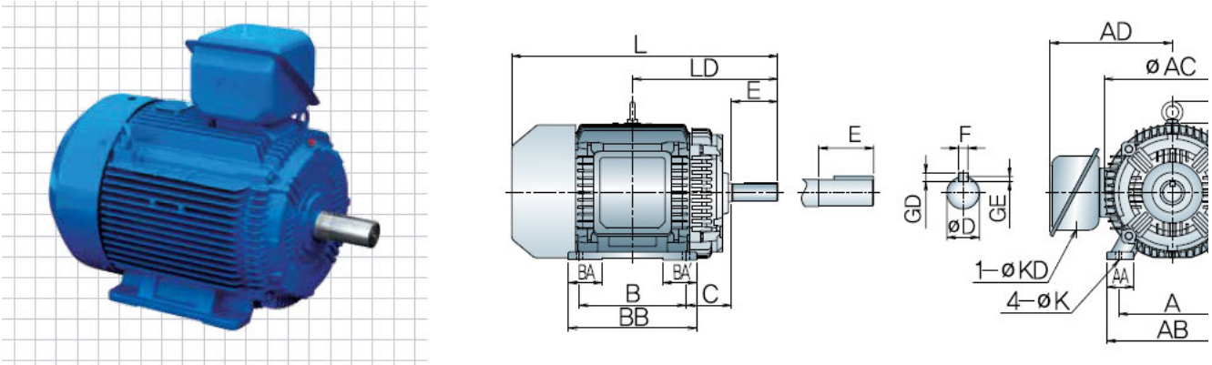
30KW / 40HP 4-pole TEFC Induction Motor, Foot Mounted
