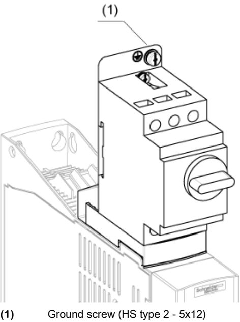
(1) Ground screw (HS type 2 - 5x12)
